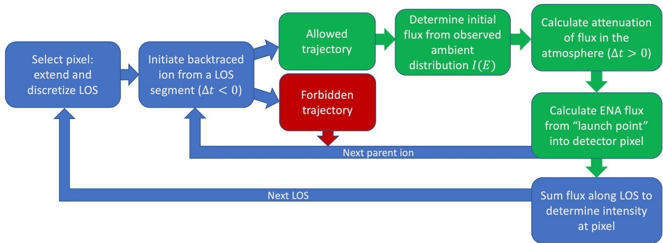
Figure 2. Logical structure of the backtracing model used to calculate synthetic ENA images at Europa and Callisto (adapted from Tippens et al. (2024)).
